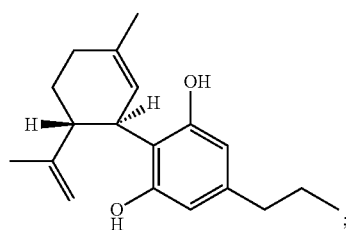
CBDV Cannabidivarin
