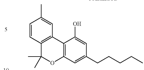
CBN Cannabinol
