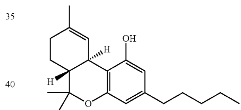
THC Tetrahydrocannabinol
