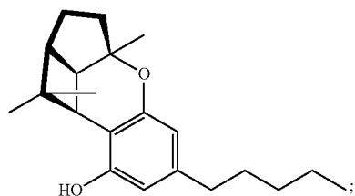
CBL Cannabicyclol
