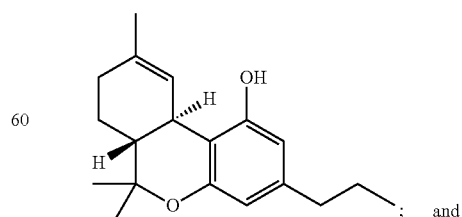
THCV Tetrahydrocannabivarin
